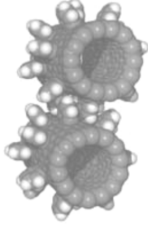
Molecular gears
